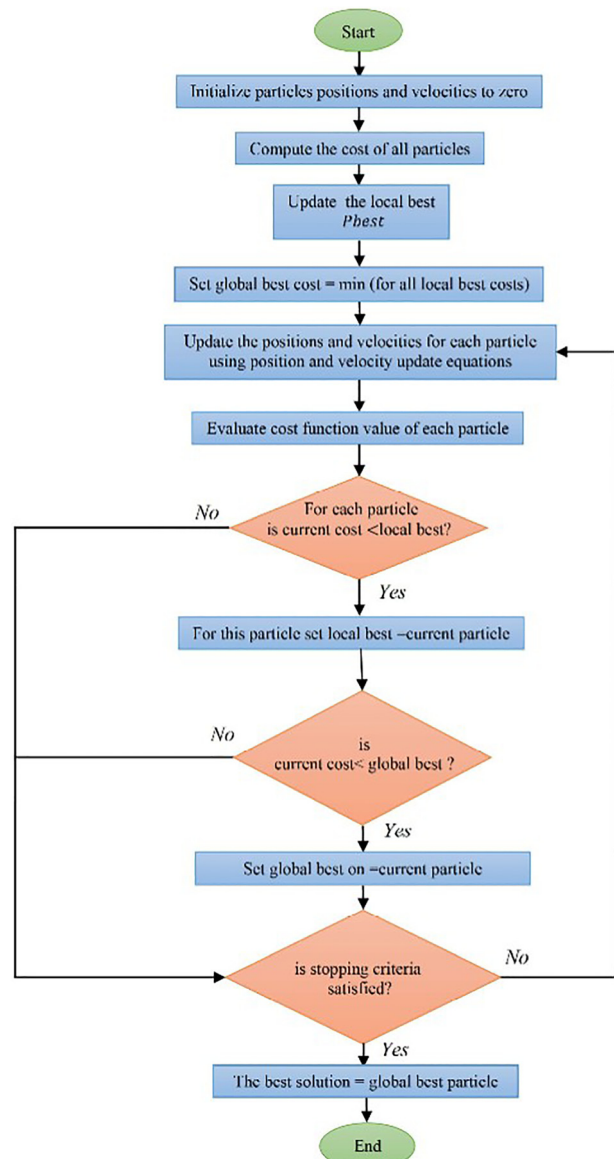
Fig. 4. PSO flowchart
