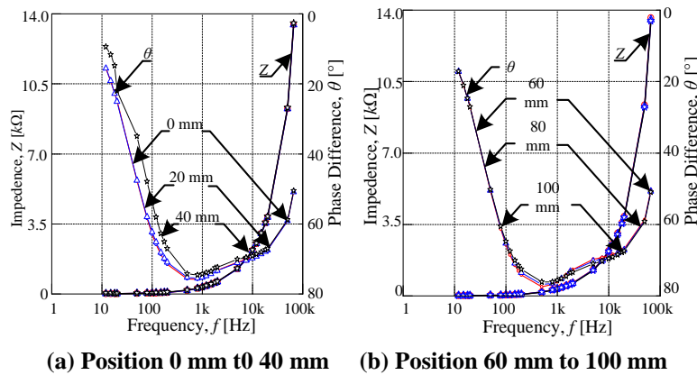
Fig. 6. Effect of frequency to the value of impedance, Z and phase difference, \theta for slot-less linear motor
