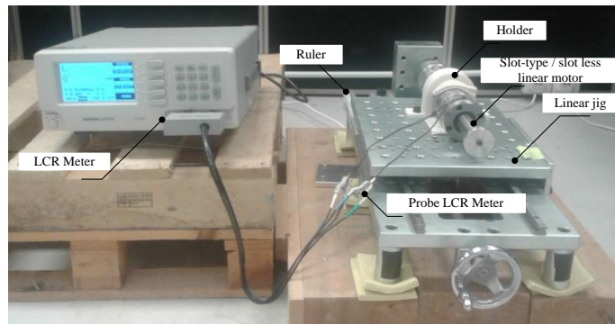
Fig. 4. Measurement setup.
