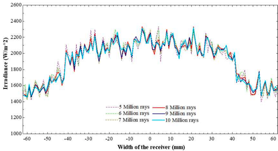
Fig. 7. Analysis of the number of rays' sensitivity.
