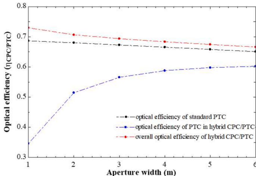
Fig. 17. Comparison of optical efficiency of standard PTC, PTC in CPC/PTC and hybrid CPC/PTC system ( 45^\circ rim angle).
