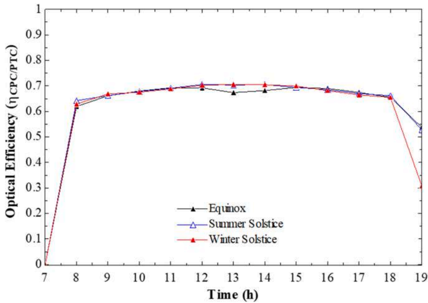
Fig. 18. Optical efficiency of hybrid CPC/PTC: dual-axis tracking.
