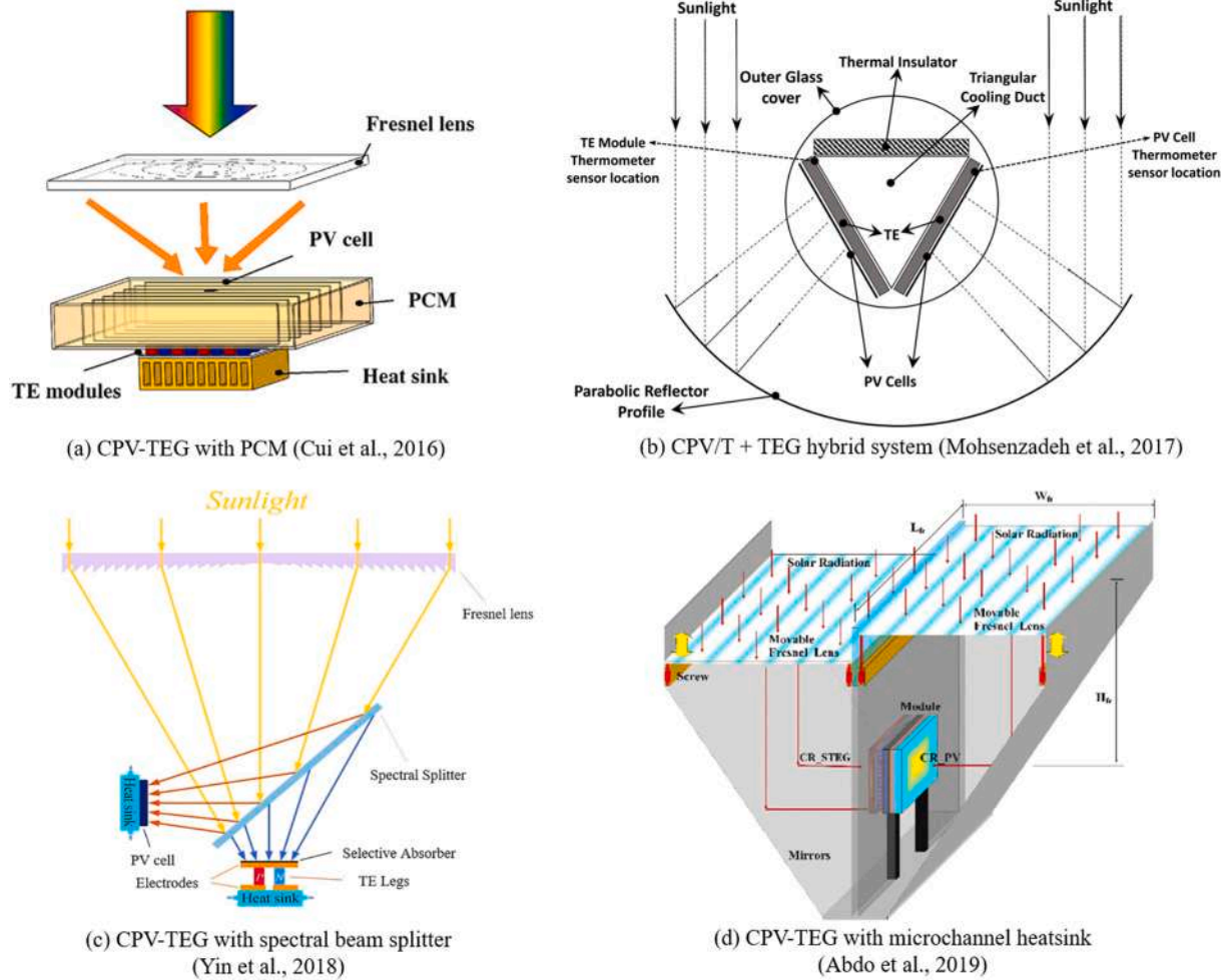
Fig. 1. Various types of solar concentrators used in hybrid CPVT-TEG system.
