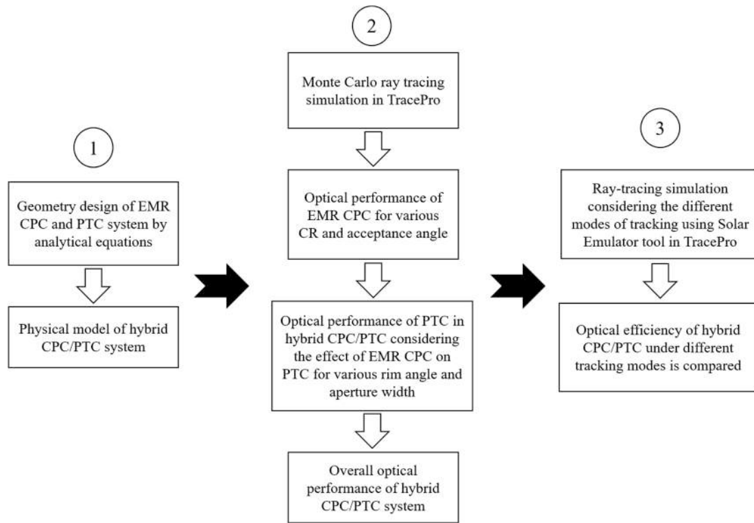
Fig. 3. Flowchart of the whole procedure for investigating the optical performance.
