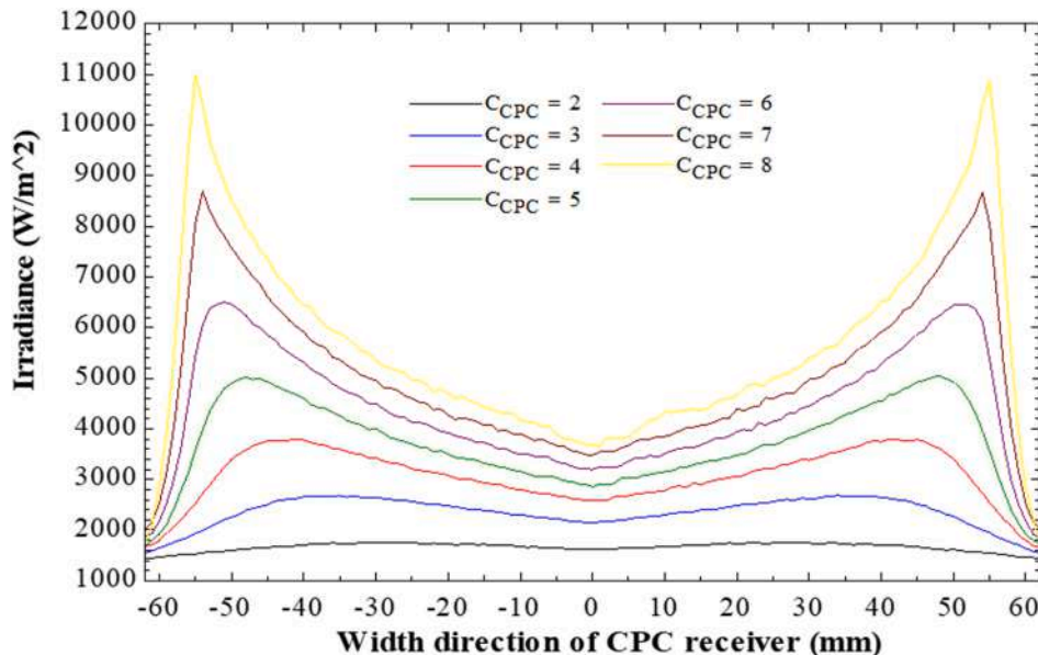
Fig. 12. Irradiance distribution of LEMR CPC.
