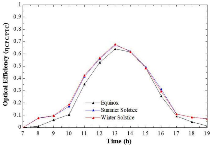
Fig. 20. Optical efficiency of hybrid CPC/PTC: N-S tracking on a horizontal E-W axis.
