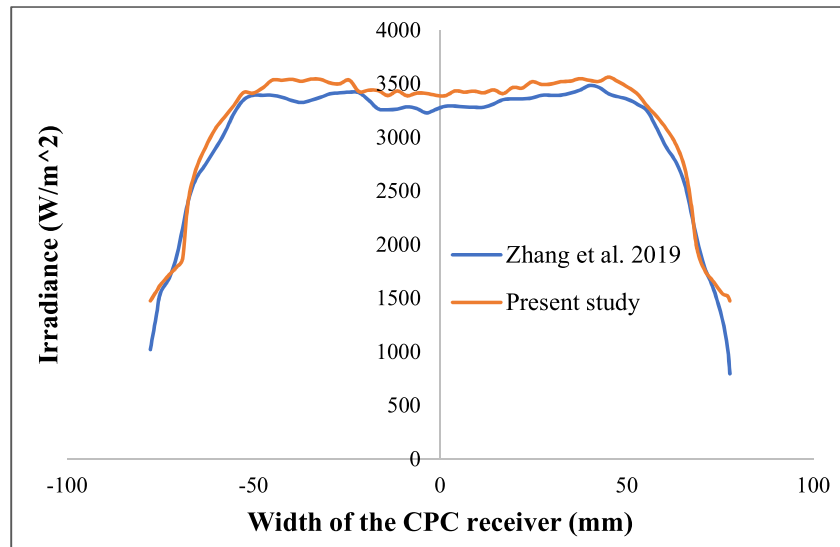
Fig. 9. The validation transversal profile of the irradiance distribution for CPC with a flat receiver.
