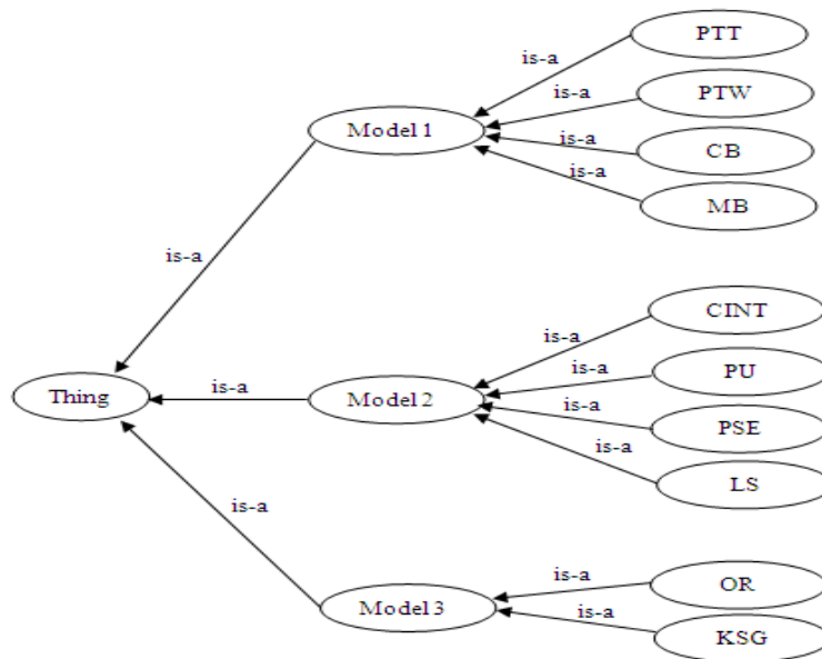
Fig. 3. Ontology structure.
