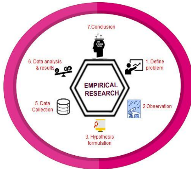
Fig. 4. Methodological framework.
