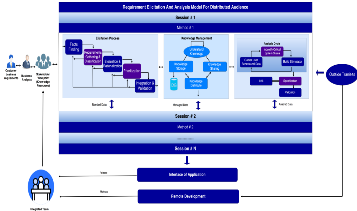
Figure 2 Requirements Elicitation and Analysis Model for the Distributed Audience
